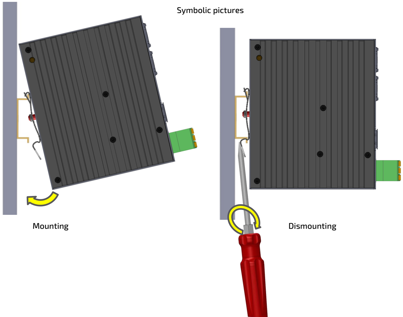
Figure 4: Mounting and dismounting a Control Unit on a DIN rail
