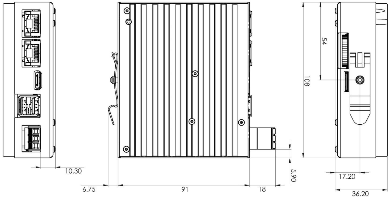
Figure 6: Views and dimensions
