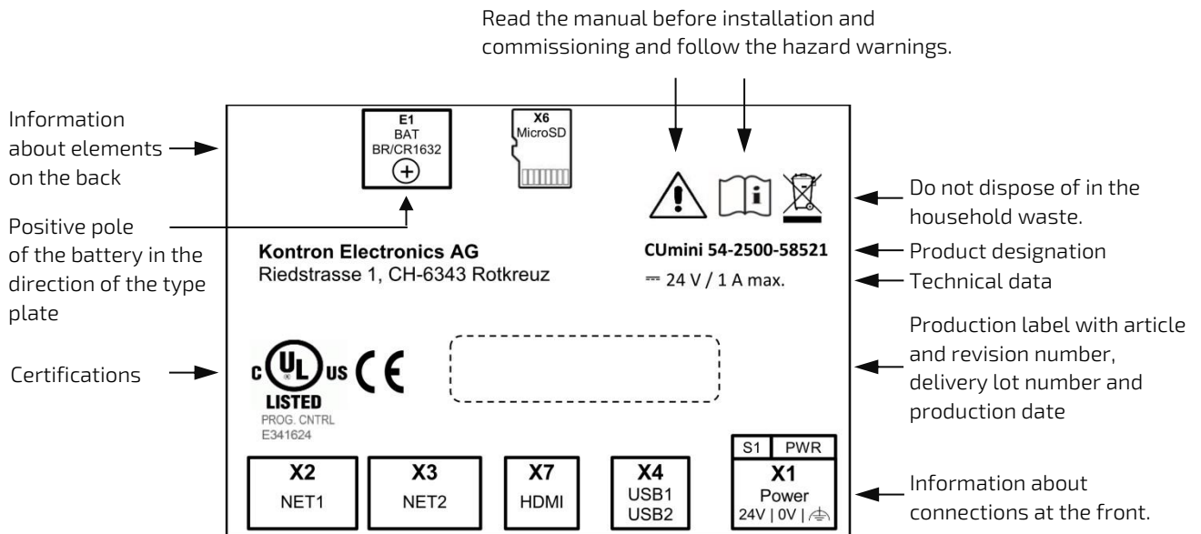
Figure 1: Type Label
