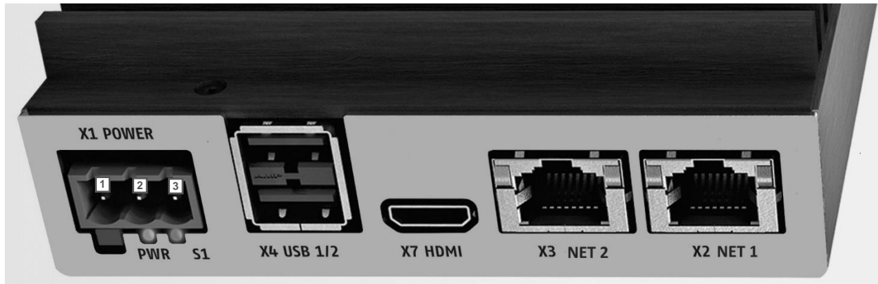
Figure 2: Interfaces/Connectors Front side
