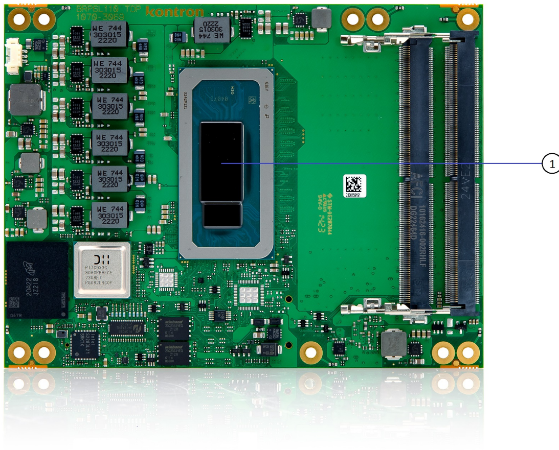
Figure 4: 1. Temperature Sensor in Processor (CPU)
