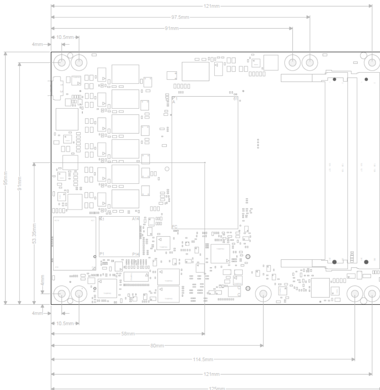
Figure 7: Module Dimensions
